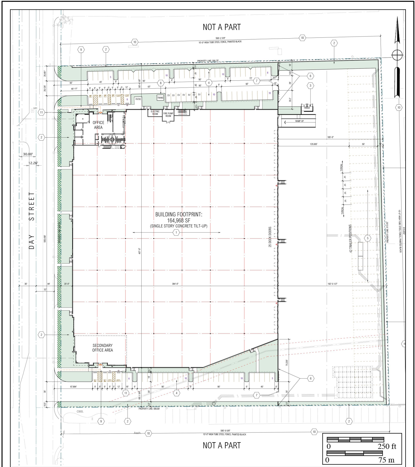
Figure 2.0-3 Site Plan
